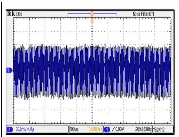
Figure 36: ERM06H100 Typical Output Ripple and Noise Vin = 110Vdc Load: I o = 6.25A Ch 1: Vo
