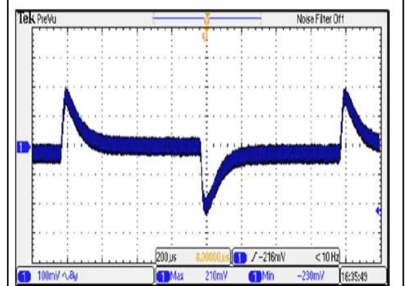
Figure 4: ERM30A100 Transient Response Vin = 50Vdc Load: Io = 100% to 75% load change Ch 1: Vo
