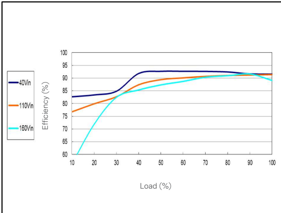
Figure 23: ERM10C100 Efficiency Versus Output Current Curve Vin = 40 to 160 Vdc Load: Io = 0 to 10 A
