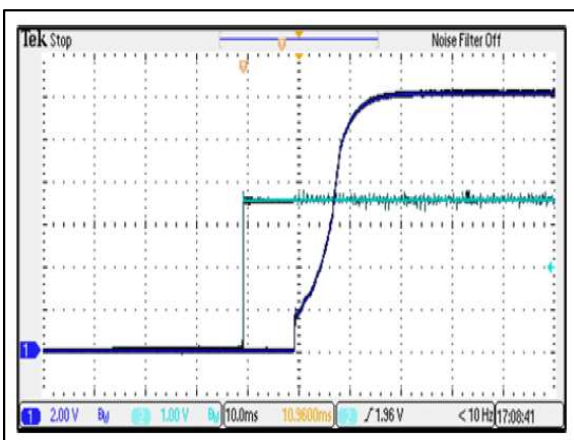
Figure 16: ERM12B100 Output Voltage Startup Characteristic by On/Off Vin = 50Vdc Load: Io = 12.5A Ch 1: Vo Ch 2: Remote On/Off
