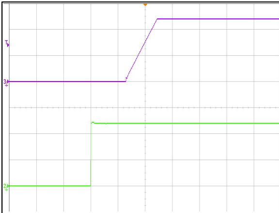
Figure 3: ADQ600B-48S12B Output Voltage Startup Characteristic Vin = 48Vdc Load: Io = 50A (50mS/div) Ch 2: Vi (20V/div) Ch 3: Vo (5V/div)
