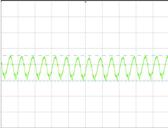
Figure 1: ADQ600B-48S12B Input Reflected Ripple Current Vin = 48Vdc Load: Io = 50A Ch 1: Iin (5uS/div, 50mA/div)
