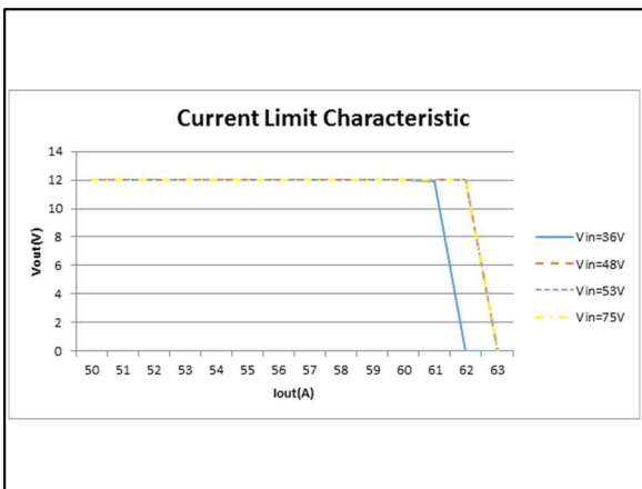
Figure 11: ADQ600B-48S12B Current Limit Characteristic
