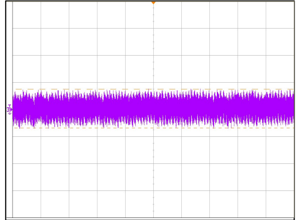
Figure 2: ADQ600B-48S12B Ripple and Noise Measurement Vin = 48Vdc Load: Io = 50A Ch 3: Vo (1ms/div, 50mV/div)
