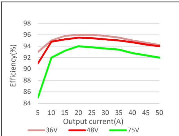
Figure 9: ADQ600B-48S12B Efficiency curve@25 degC Loading: Io=5~50A
