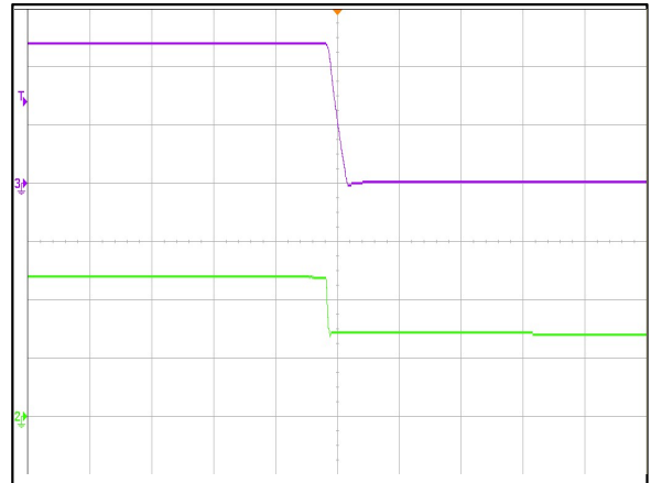
Figure 4: ADQ600B-48S12B Turn Off Characteristic (5mS/div) Vin = 48Vdc Load: Io = 50A Ch 2: Vi (20V/div) Ch 3: Vo (5V/div)
