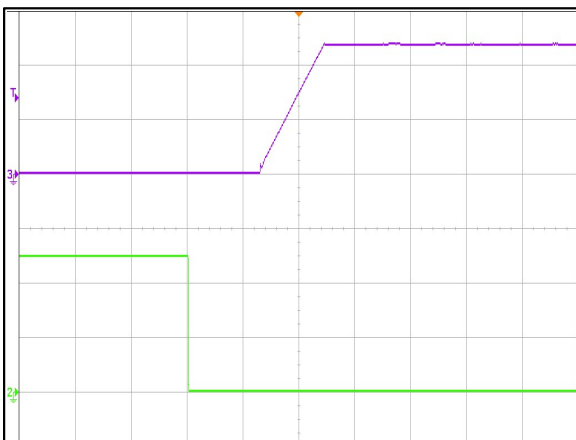
Figure 5: ADQ600B-48S12B Remote ON Waveform (50mS/div) Vin = 48Vdc Load: Io = 50A Ch 2: Remote ON (2V/div) Ch 3: Vo (5V/div)
