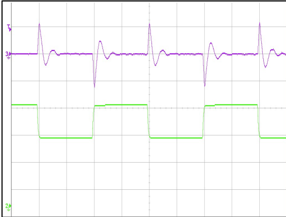
Figure 7: ADQ600B-48S12B Transient Response (2mS/div) 50%-75%-50% load change, 0.1A/uS slew rate, Vin = 48Vdc Ch 2: Io (10A/div) Ch 4: Vo (200mV/div)
