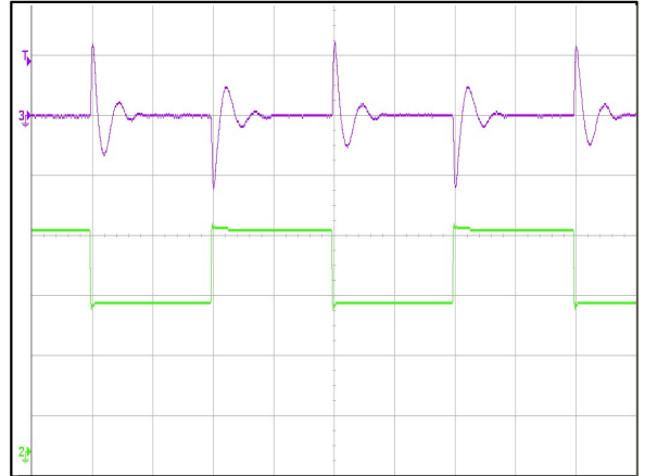
Figure 8: ADQ600B-48S12B Transient Response (2mS/div) 50%-75%-50% load change, 1A/uS slew rate, Vin = 48Vdc Ch 2: Io (10A/div) Ch 4: Vo (200mV/div)
