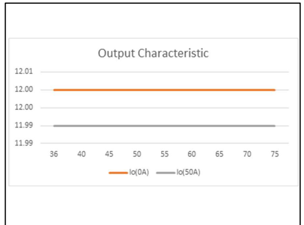
Figure 10: ADQ600B-48S12B Output Characteristic Loading: Io=0~50A
