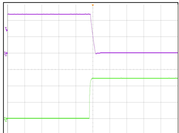
Figure 6: ADQ600B-48S12B Remote OFF Waveform (5mS/div) Vin = 48Vdc Load: Io = 50A Ch 2: Remote OFF (2V/div) CH3: Vo (5V/div)
