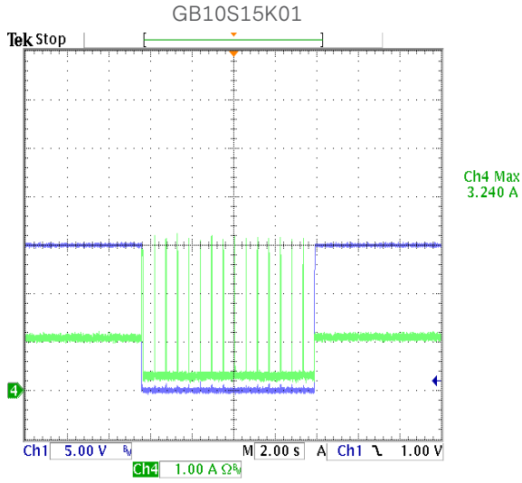
Figure 48: Output Over Load at 90Vac
