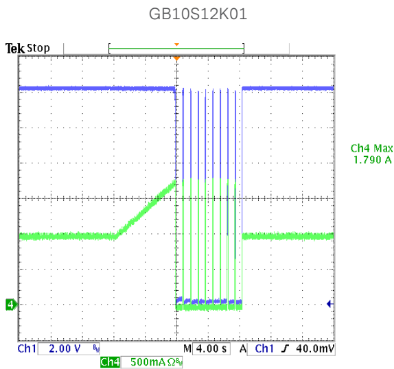
Figure 38: Output Over Load at 90Vac CH1: Vout CH4: Over Load Current
