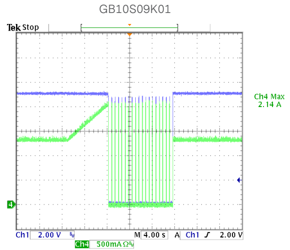
Figure 37: Output Over Load at 264Vac CH1:Vout CH4: Over Load Current
