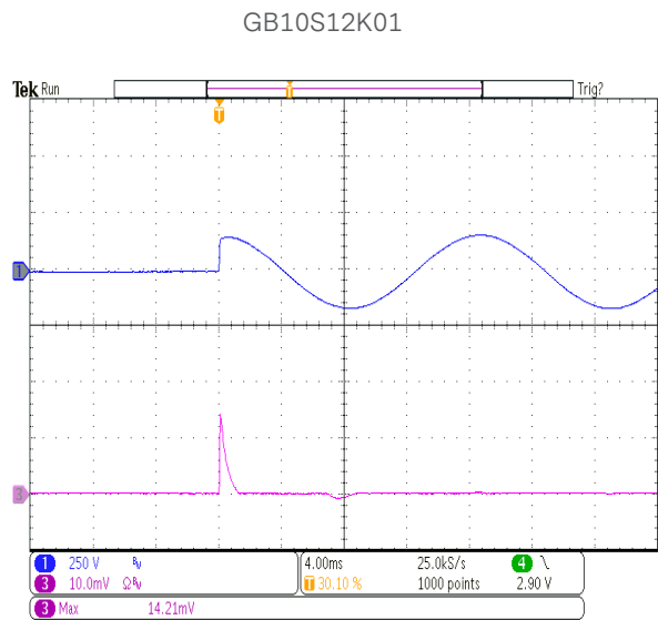
Figure 6: Inrush Current at 115Vac 12V/1A - CH3: 10A/Div I(\text{inrush}) = 14.21\text{A peak} I^2t = 0.13\text{A}^2\text{S}
