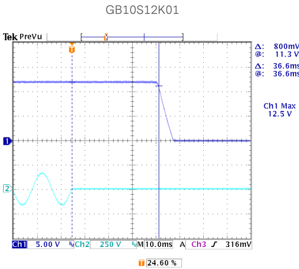
Figure 30: Turn-on rise time at 115Vac - 1.0A load
