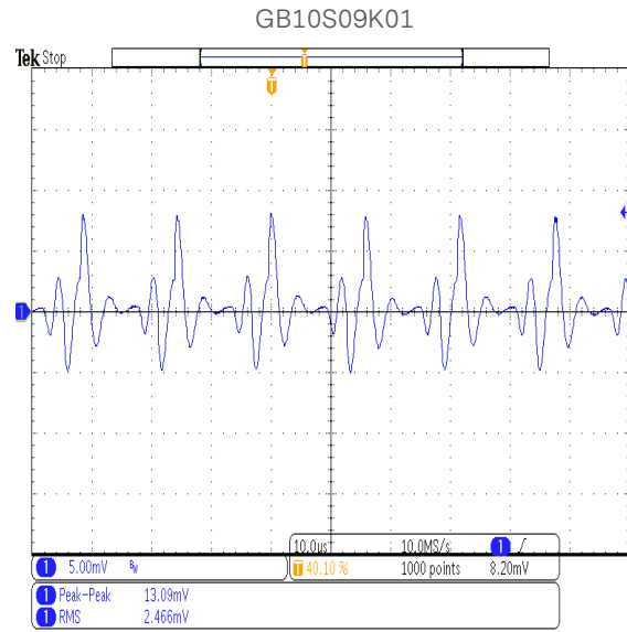
Figure 61: Common Mode Current at 230Vac Current Probe:1mA/mV
