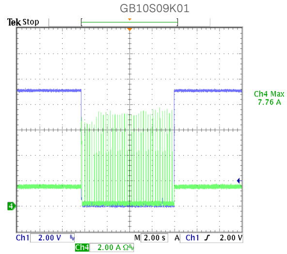
Figure 45: Output Over Load at 264Vac
