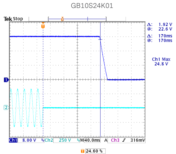
Figure 35: Tutn-on rise time at 230Vac - 0.5A load
