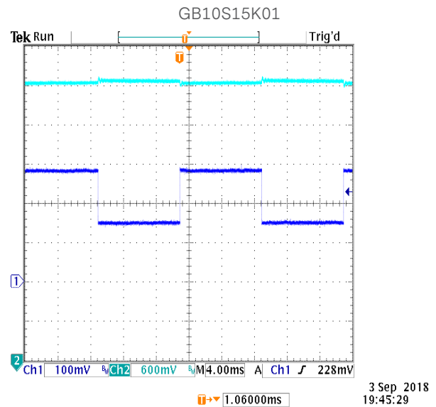
Figure 57: Transient Response at 230Vac, 50%-100% step load CH1:Vout CH4: Load Current
