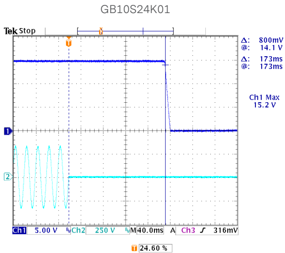
Figure 34: Tutn-on rise time at 115Vac - 0.5A load
