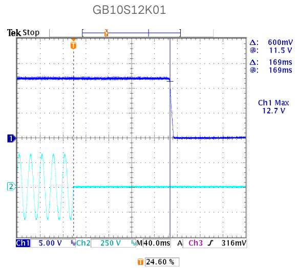
Figure 31: Turn-on rise time at 230Vac - 1.0A load
