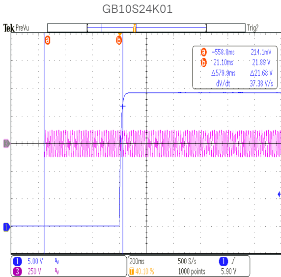
Figure 18: Turn-on delay at 90Vac - 0.5A load
