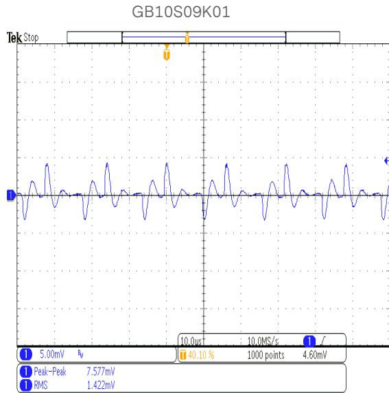
Figure 60: Common Mode Current at 115Vac Current Probe:1mA/mV
