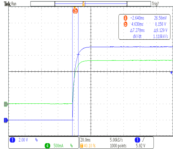
Figure 21: Turn-on rise time at 264Vac - 1.33A load
