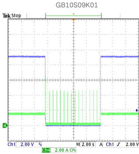
Figure 44: Output Over Load at 90Vac
