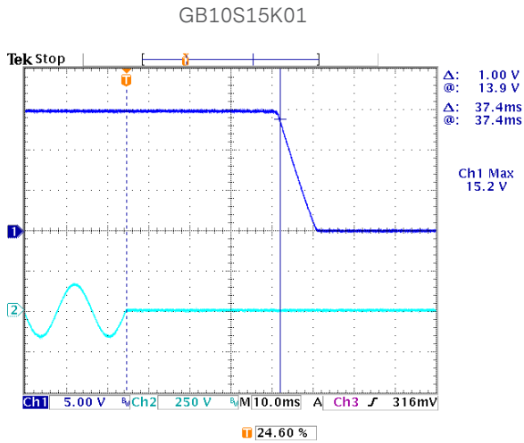
Figure 32: Hold-up time at 115Vac - 0.8A load
