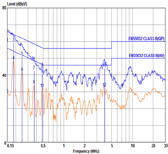
Figure 75: EN55032 CLASS B – 230V/60Hz 100% Load margin >10 dB. Blue Plot: Quasi-Peak. Red Plot: Average.
