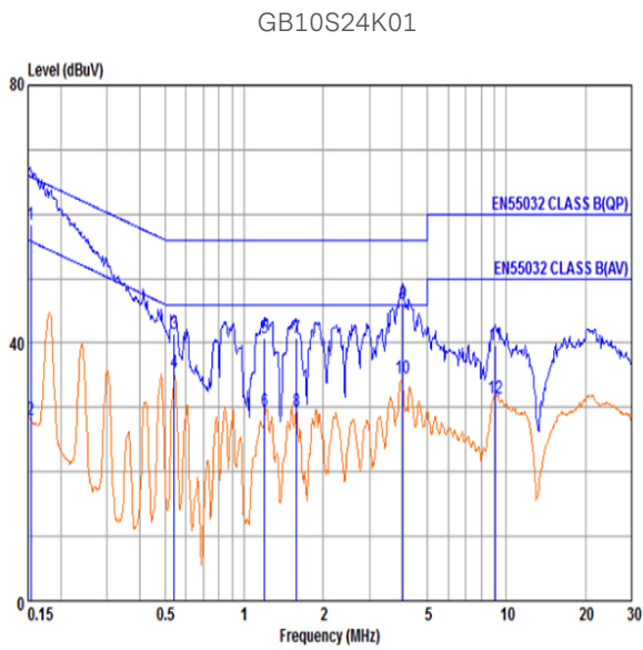
Figure 71: EN55032 CLASS B – 230V/60Hz 100% Load margin >10 dB. Blue Plot: Quasi-Peak. Red Plot: Average.
