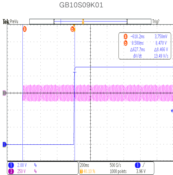
Figure 12: Turn-on delay at 90Vac - 1.33A load
