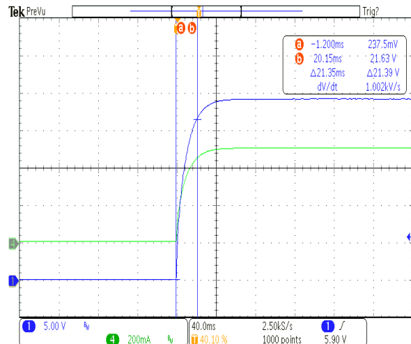
Figure 27: Turn-on rise time at 264Vac - 0.5A load
