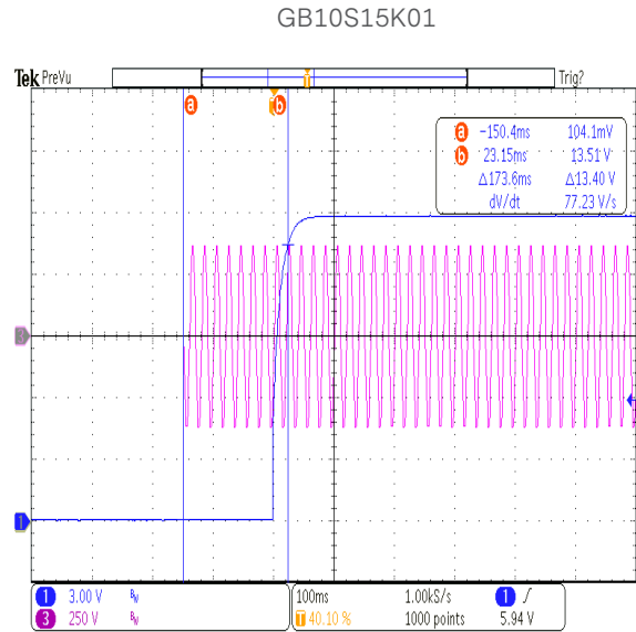
Figure 17: Turn-on delay at 264Vac - 0.8A load
