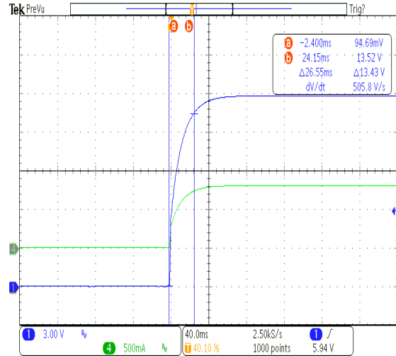
Figure 25: Turn-on rise time at 264Vac - 0.8A load
