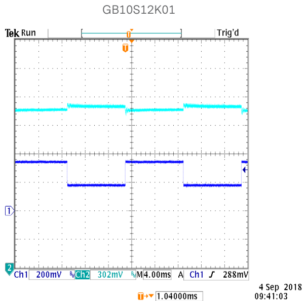
Figure 55: Transient Response at 230Vac, 50%-100% step load CH1:Vout CH4: Load Current
