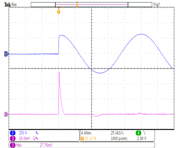
Figure 11: Inrush Current at 230Vac 24V/0.5A - CH3: 10A/Div I(\text{inrush}) = 27.76\text{A peak} I^2t = 0.55\text{A}^2\text{S}
