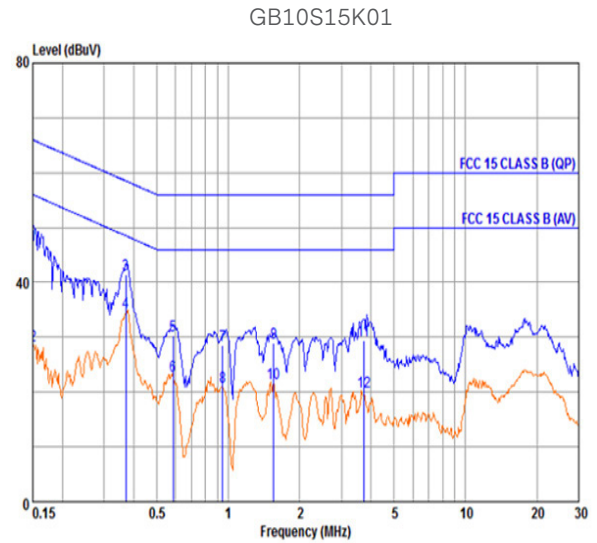
Figure 78: EN55032 CLASS B – 120V/60Hz 10% Load magin >10 dB Blue Plot: Quasi-Peak. Red Plot: Average.
