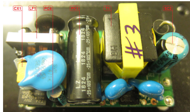
Figure 2: PCB Mount Type
