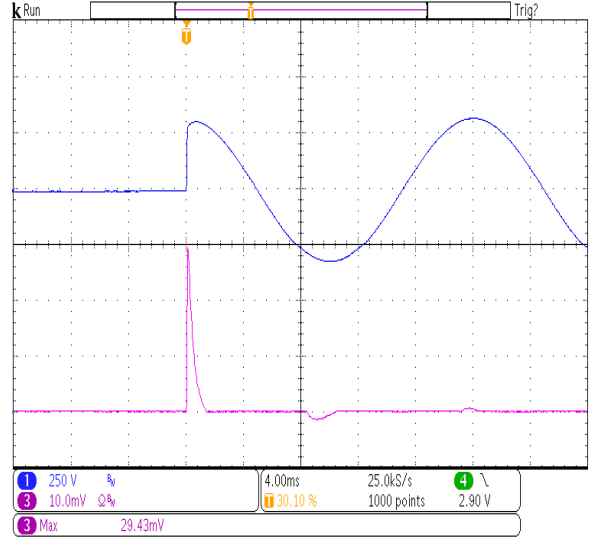
Figure 9: Inrush Current at 230Vac 15V/0.8A - CH3: 10A/Div I(\text{inrush}) = 27.38\text{A peak} I^2t = 0.54\text{A}^2\text{S}
