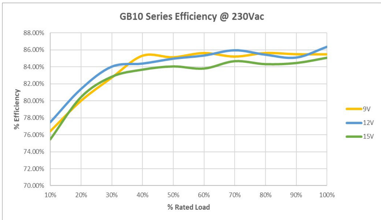
Fig. 68: GB10 Series Efficiency Curves.
