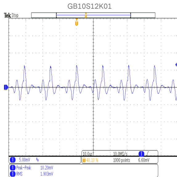
Figure 63: Common Mode Current at 230Vac Current Probe:1mA/mV
