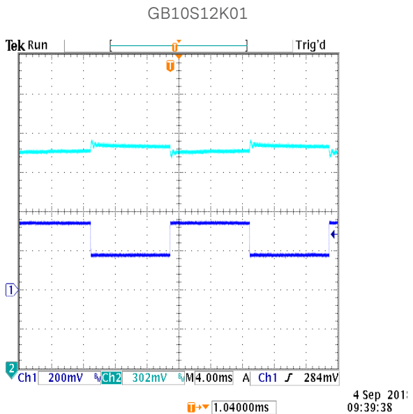
Figure 54: Transient Response at 115Vac, 50%-100% step load CH1: Vout CH4: Load Current
