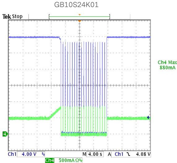
Figure 43: Output Over Load at 264Vac CH1:Vout CH4: Over Load Current
