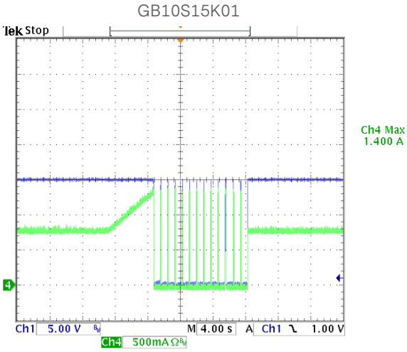
Figure 40: Output Over Load at 90Vac CH1: Vout CH4: Over Load Current
