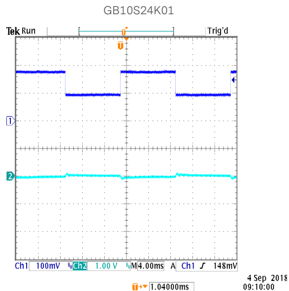
Figure 58: Transient Response at 115Vac, 50%-100% step load CH1: Vout CH4: Load Current
