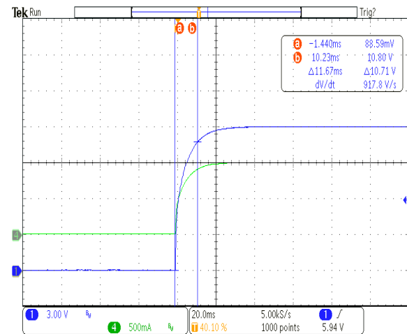
Figure 23: Turn-on rise time at 264Vac - 1.0A load
