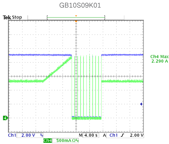
Figure 36: Output Over Load at 90Vac CH1: Vout CH4: Over Load Current
