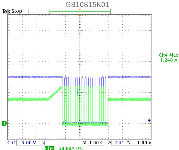
Figure 41: Output Over Load at 264Vac CH1:Vout CH4: Over Load Current
