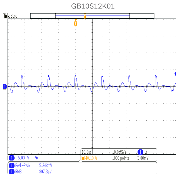
Figure 62: Common Mode Current at 115Vac Current Probe:1mA/mV
