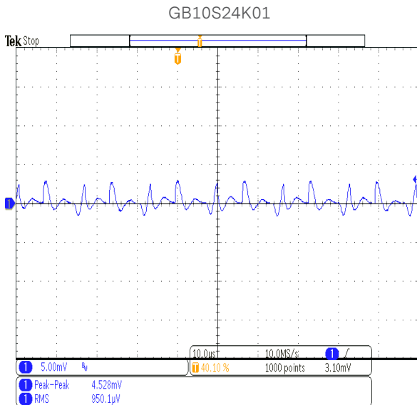
Figure 66: Common Mode Current at 115Vac Current Probe:1mA/mV
