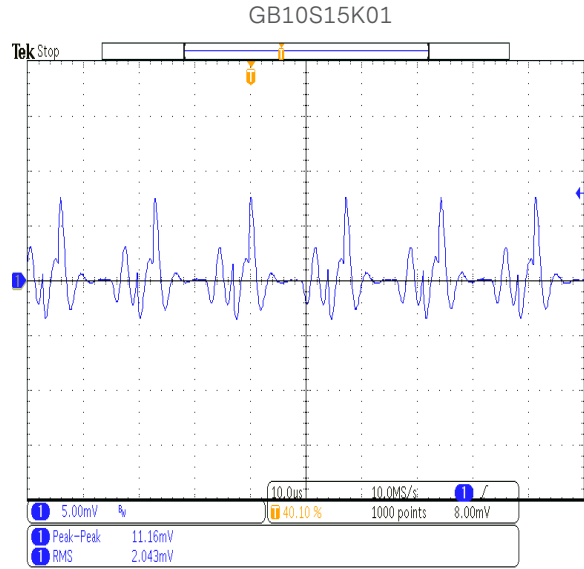
Figure 65: Figure 60: Common Mode Current at 230Vac Current Probe:1mA/mV
