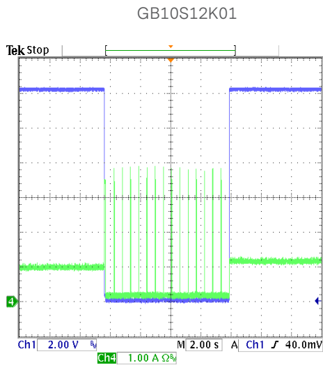
Figure 46: Output Over Load at 90Vac
