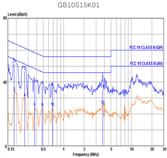
Figure 77: EN55032 CLASS B – 120V/60Hz 100% Load magin >10 dB. Blue Plot: Quasi-Peak. Red Plot: Average.
