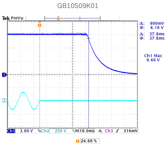
Figure 28: Hold-up time at 115Vac - 1.33A load
