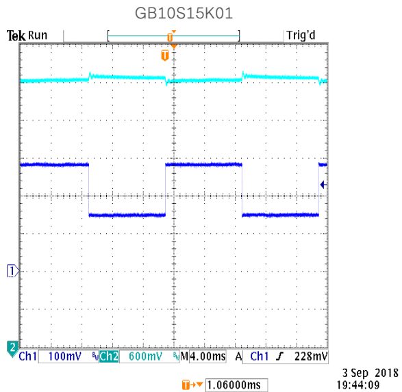
Figure 56: Transient Response at 115Vac, 50%-100% step load CH1: Vout CH4: Load Current
