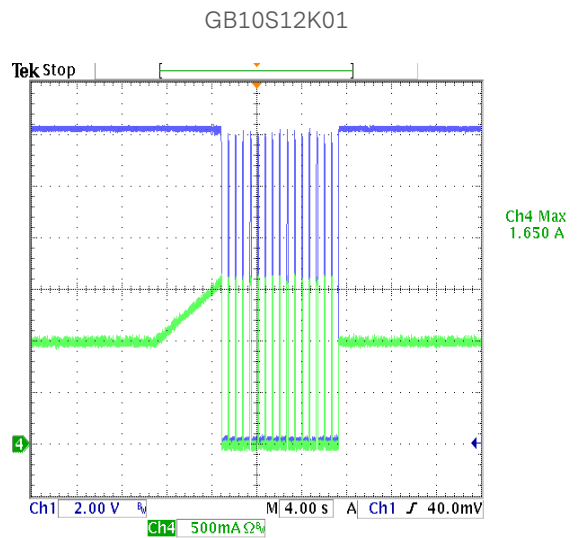
Figure 39: Output Over Load at 264Vac CH1:Vout CH4: Over Load Current
