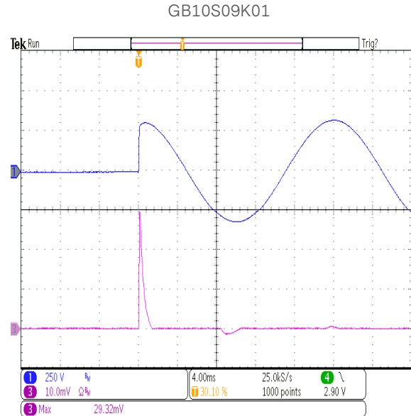
Figure 5: Inrush Current at 230Vac 9V/1.33A - CH3: 10A/Div I(\text{inrush}) = 29.31\text{A peak} I^2t = 0.60\text{A}^2\text{S}
