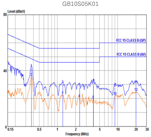
Figure 70: EN55032 CLASS B – 120V/60Hz 10% Load margin >10 dB Blue Plot: Quasi-Peak. Red Plot: Average.
