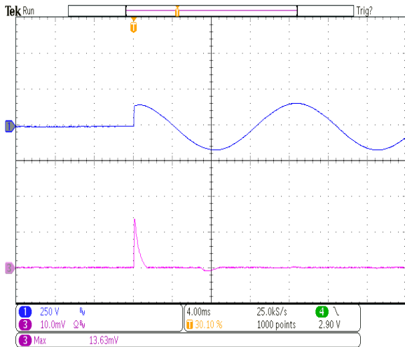
Figure 10: Inrush Current at 115Vac 24V/0.5A - CH3: 10A/Div I(\text{inrush}) = 13.63\text{A peak} I^2t = 0.13\text{A}^2\text{S}
