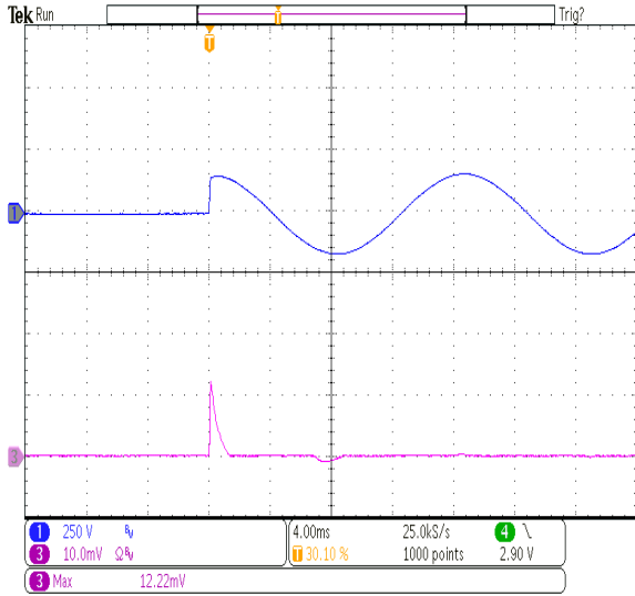
Figure 8: Inrush Current at 115Vac 15V/0.8A - CH3: 10A/Div I(\text{inrush}) = 12.22\text{A peak} I^2t = 0.11\text{A}^2\text{S}
