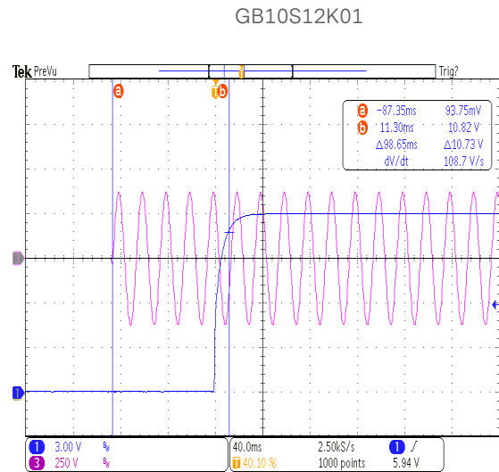
Figure 15: Turn-on delay at 264Vac - 1.0A load
