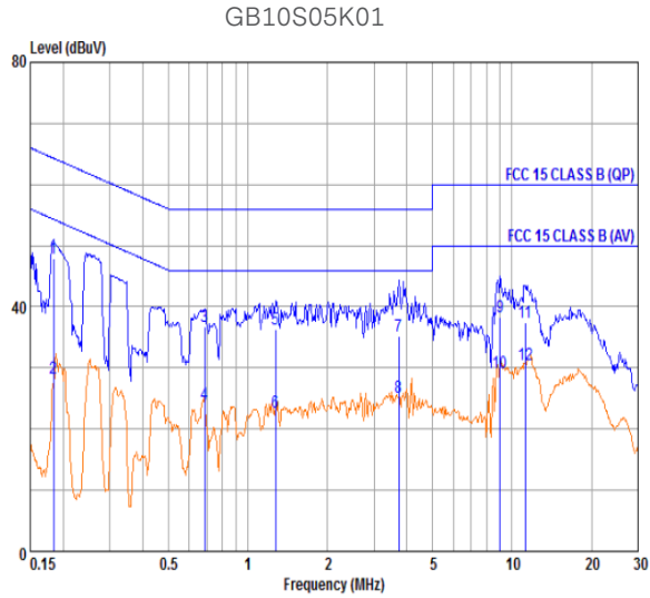
Figure 69: EN55032 CLASS B – 120V/60Hz 100% Load margin >10 dB. Blue Plot: Quasi-Peak. Red Plot: Average.
