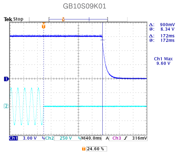
Figure 29: Hold-up time at 230Vac - 1.33A load
