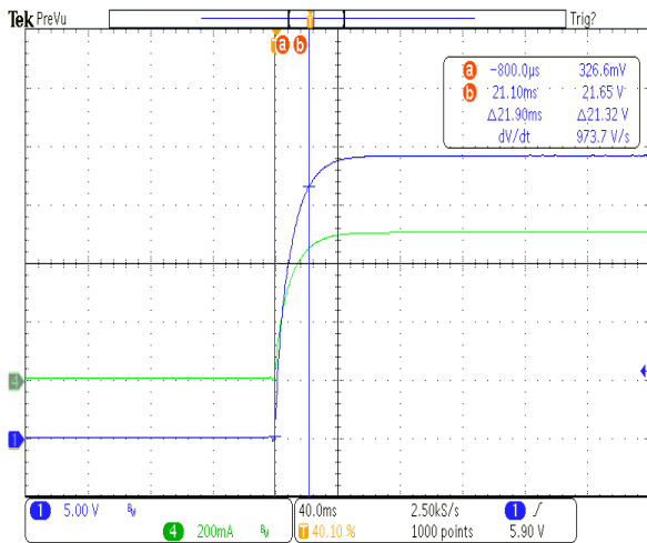
Figure 26 Turn-on rise time at 90Vac - 0.5A load
