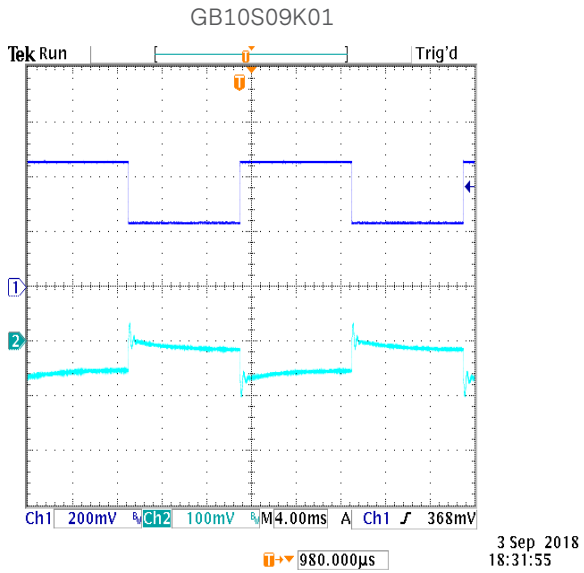
Figure 52: Transient Response at 115Vac, 50%-100% step load CH1: Vout CH4: Load Current
