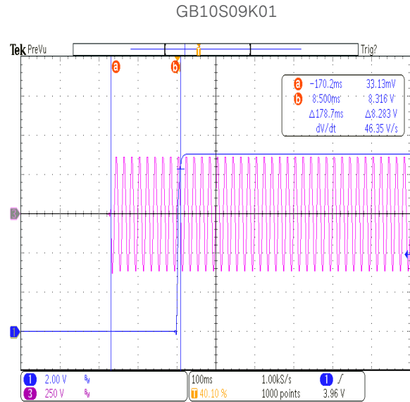
Figure 13: Turn-on delay at 264Vac - 1.33A load
