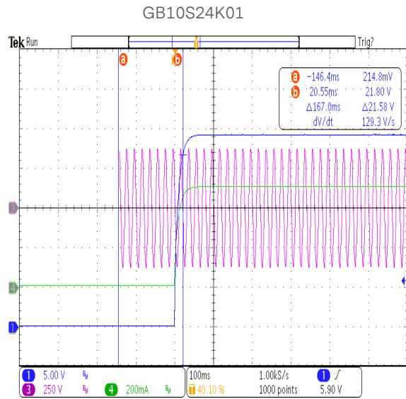
Figure 19: Turn-on delay at 264Vac - 0.5A load
