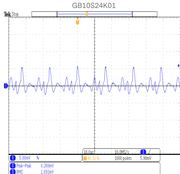
Figure 67: Common Mode Current at 230Vac Current Probe:1mA/mV
