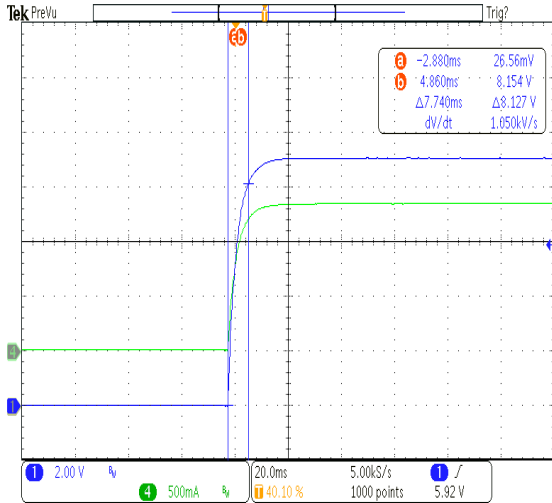
Figure 20: Turn-on rise time at 90Vac - 1.33A load
