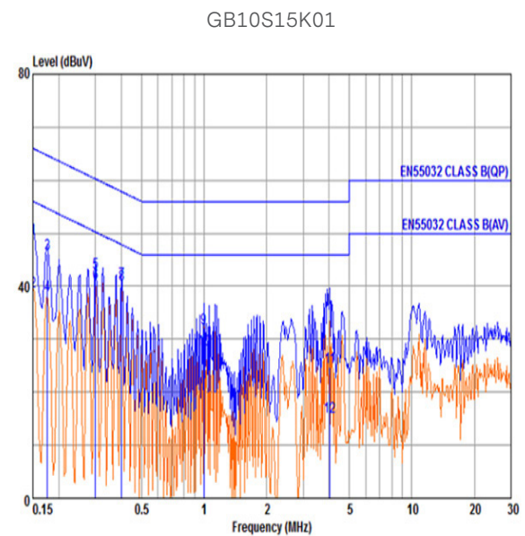
Figure 80: EN55032 CLASS B – 230V/60Hz 10% Load magin >10 dB Blue Plot: Quasi-Peak. Red Plot: Average.
