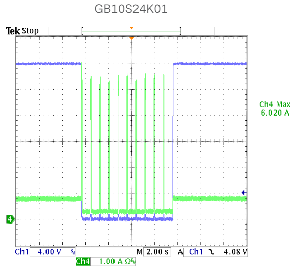
Figure 51: Output Over Load at 264Vac
