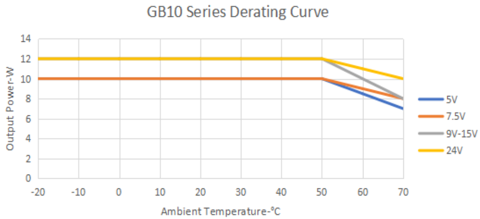
Figure 3: GB10 Series Derating Curve
