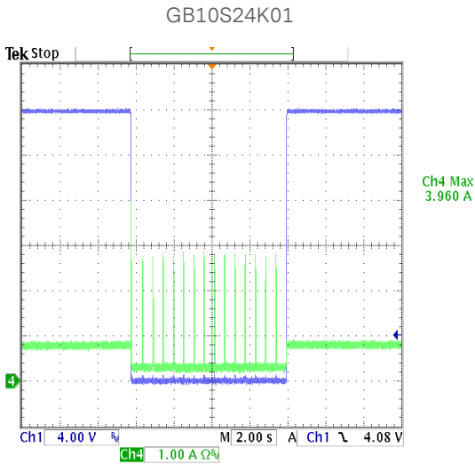
Figure 50: Output Over Load at 90Vac
