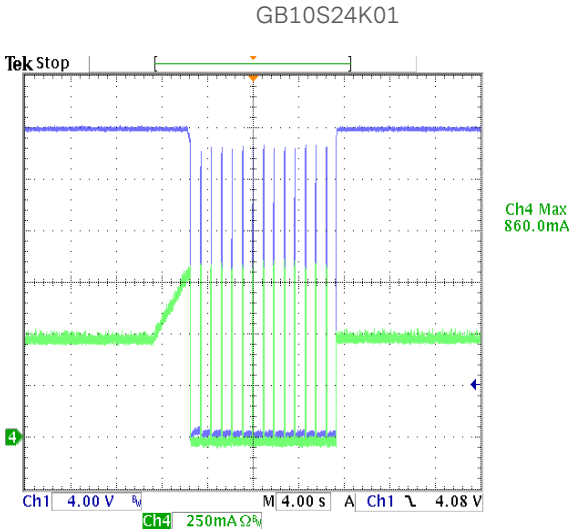
Figure 42: Output Over Load at 90Vac CH1: Vout CH4: Over Load Current
