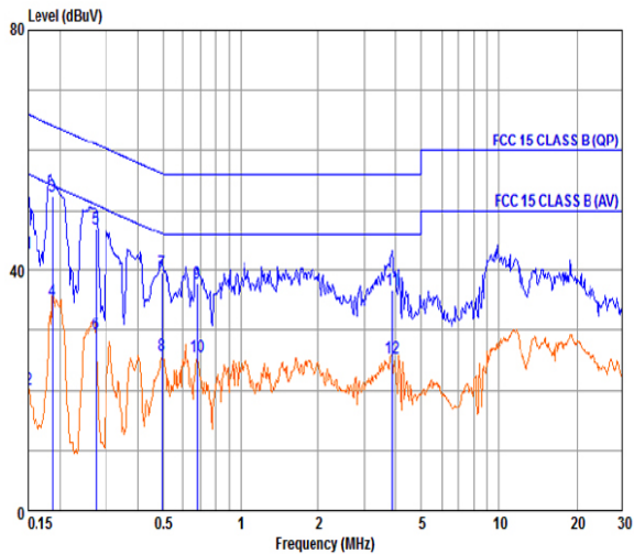
Figure 73: EN55032 CLASS B – 120V/60Hz 100% Load margin >10 dB. Blue Plot: Quasi-Peak. Red Plot: Average.
