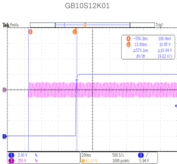
Figure 14: Turn-on delay at 90Vac - 1.0A load
