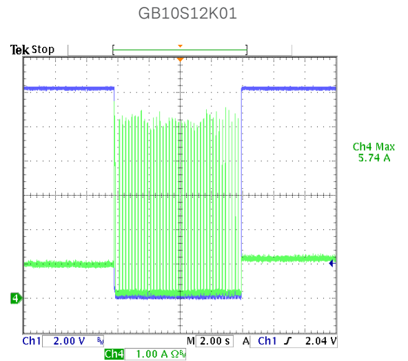
Figure 47: Output Over Load at 264Vac
