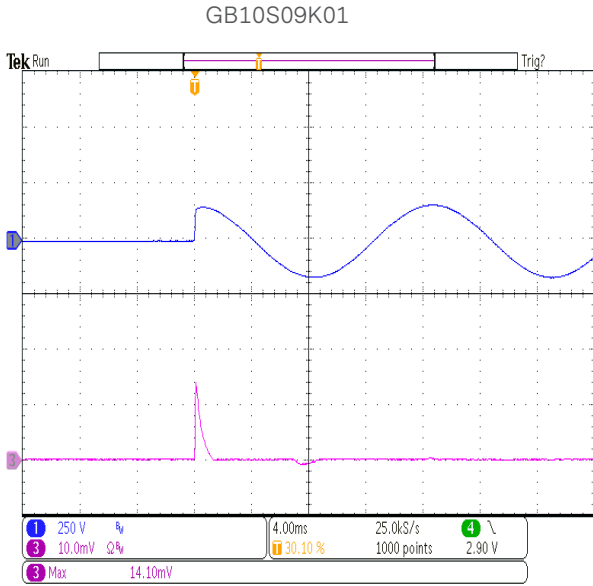
Figure 4: Inrush Current at 115Vac 9V/1.33A - CH3: 10A/Div I(\text{inrush}) = 14.1\text{A peak} I^2t = 0.13\text{A}^2\text{S}
