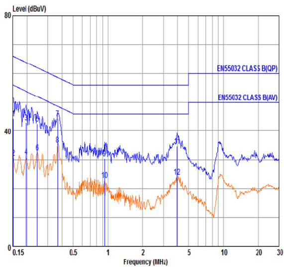
Figure 76: EN55032 CLASS B – 230V/60Hz 10% Load margin >10 dB Blue Plot: Quasi-Peak. Red Plot: Average.
