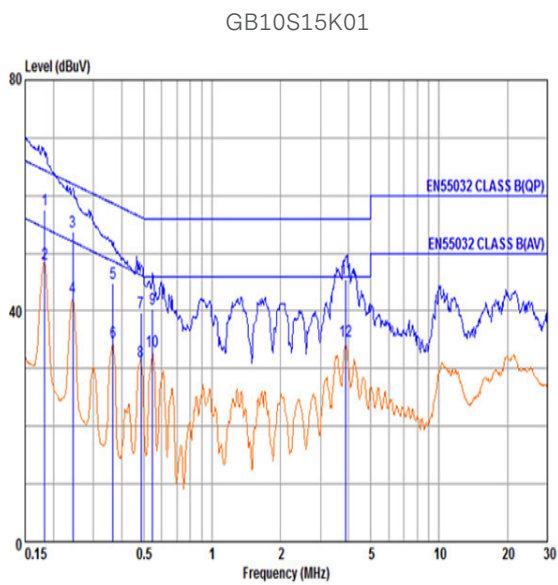
Figure 79: EN55032 CLASS B – 230V/60Hz 100% Load magin >10 dB. Blue Plot: Quasi-Peak. Red Plot: Average.
