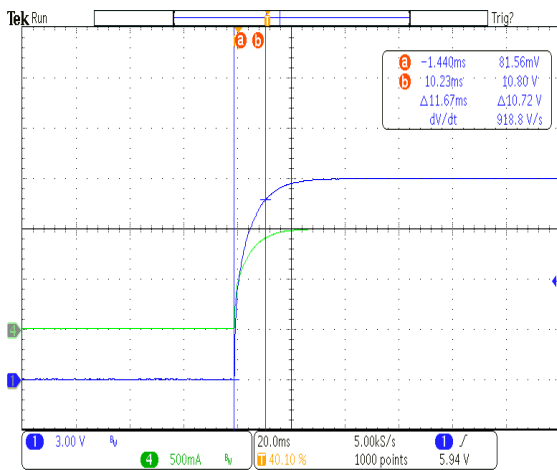
Figure 22: Turn-on rise time at 90Vac - 1.0A load
