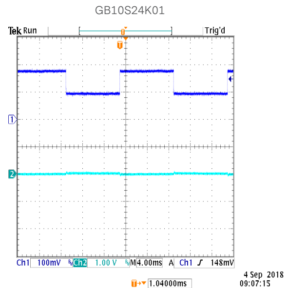
Figure 59: Transient Response at 230Vac, 50%-100% step load CH1:Vout CH4: Load Current
