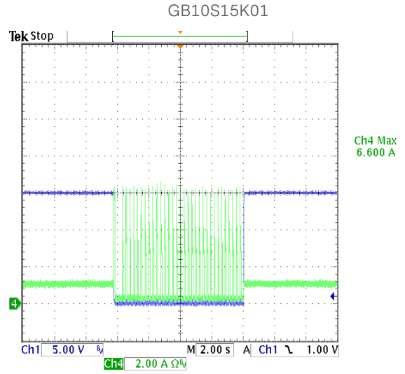
Figure 49: Output Over Load at 264Vac
