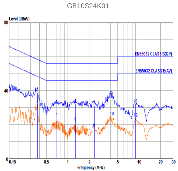
Figure 72: EN55032 CLASS B – 230V/60Hz 10% Load margin >10 dB Blue Plot: Quasi-Peak. Red Plot: Average.
