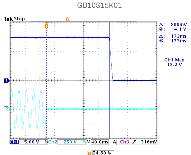
Figure 33: Hold-up time at 230Vac - 0.8A load
