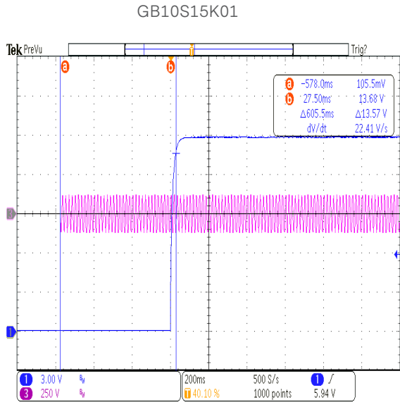
Figure 16: Turn-on delay at 90Vac - 0.8A load
