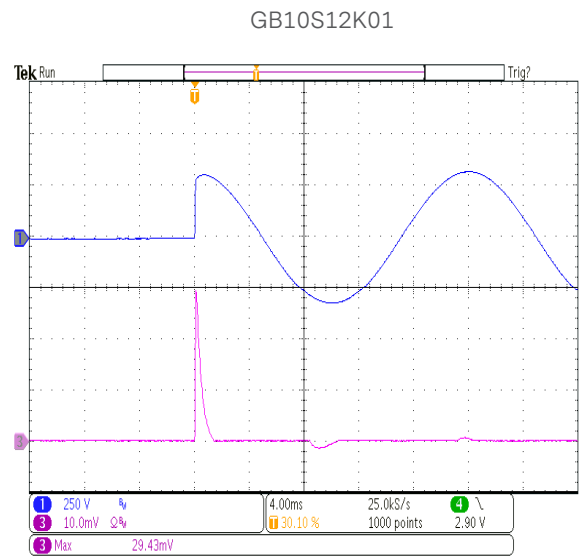
Figure 7: Inrush Current at 230Vac 12V/1A - CH3: 10A/Div I(\text{inrush}) = 29.43\text{A peak} I^2t = 0.60\text{A}^2\text{S}
